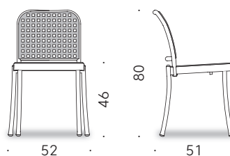
Stackable armless chair.
